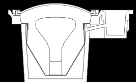
CROSS SECTION
