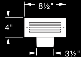
LOUVERED FACE
