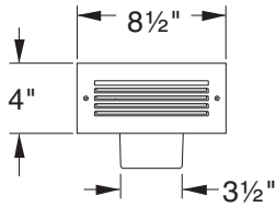
LOUVERED FACE
