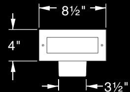
OPEN FACE
