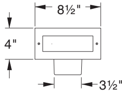
OPEN FACE
