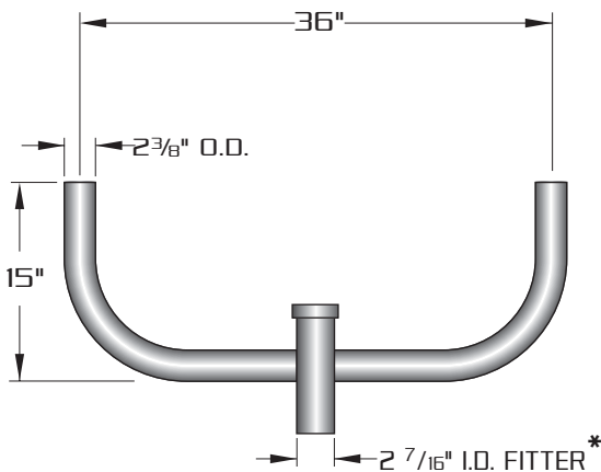
[ALUMINUM=ABH-2-180] [STEEL=SBH-2-180] E.P.A.= 0.81
