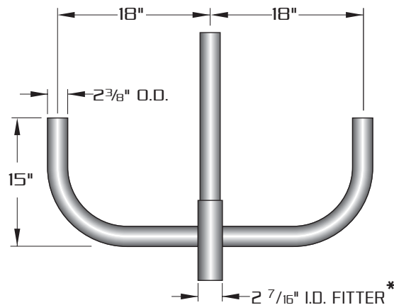
[ALUMINUM=ABH-3-180] [STEEL=SBH-3-180] E.P.A.= 1.04
