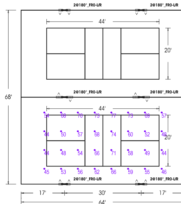
Double Court 68' x 64'
