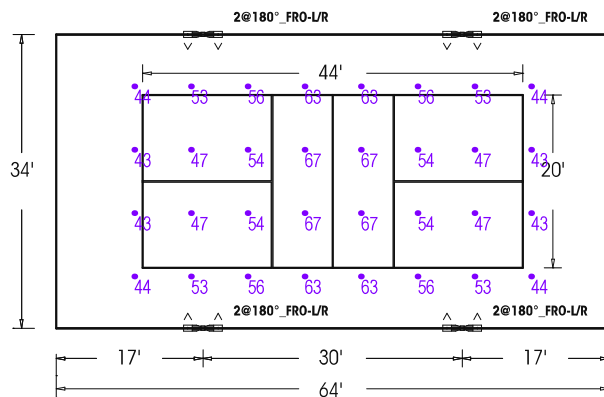
Single Court 34' x 64'
