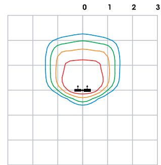
TYPE IV-CL @ 20' 5° Pivot Tilt (PT5°) FRO-R & FRO-L
