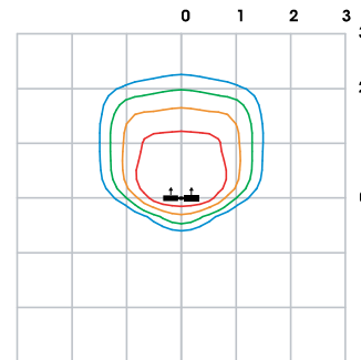
TYPE IV-CL @ 20' 5° Pivot Tilt (PT5°) FRO-R & FRO-L
