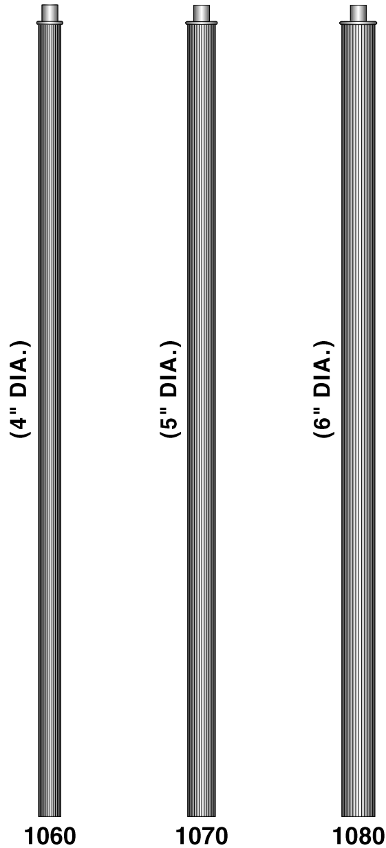
(FLUTED ALUMINUM SHAFTS) SHAFT WALL THICKNESS .188
