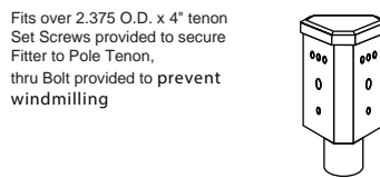
Fits over 2.375 O.D. x 4" tenon Set Screws provided to secure Fitter to Pole Tenon, thru Bolt provided to prevent windmilling T3120 Top 3 Way Fitter Adaptor
