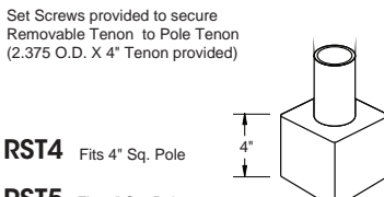
PT23 2.375 O.D. X 4" Tenon Pole Tenon
