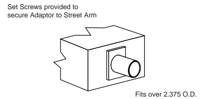
Set Screws provided to secure Adaptor to Street Arm ST23 Street Arm Adaptor
