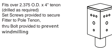
Fits over 2.375 O.D. x 4" tenon (drilled as required) Set Screws provided to secure Fitter to Pole Tenon, thru Bolt provided to prevent windmilling T490 Top 4 Way Fitter Adaptor
