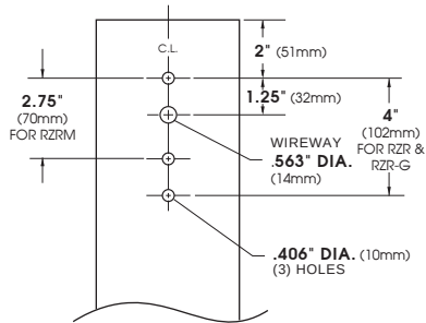
RZR-G Max Weight = 43lbs Max EPA = 0.76 120 LED Max
