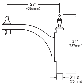
XBZ27-PM-UP-1 EPA = 1.12
