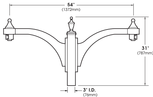
XBZ27-PM-UP-2-180 EPA = 1.23
