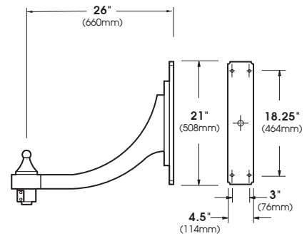
XBZ27-PM-DN-WM EPA = 0.83
