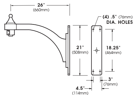
XBZ27-PM-UP-WM EPA = 0.83
